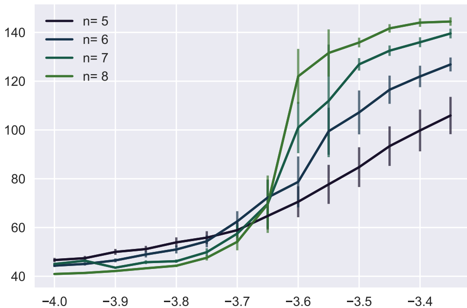
Planck Normalised Volumes (s=0.5) for type 13 scaled by d=1
