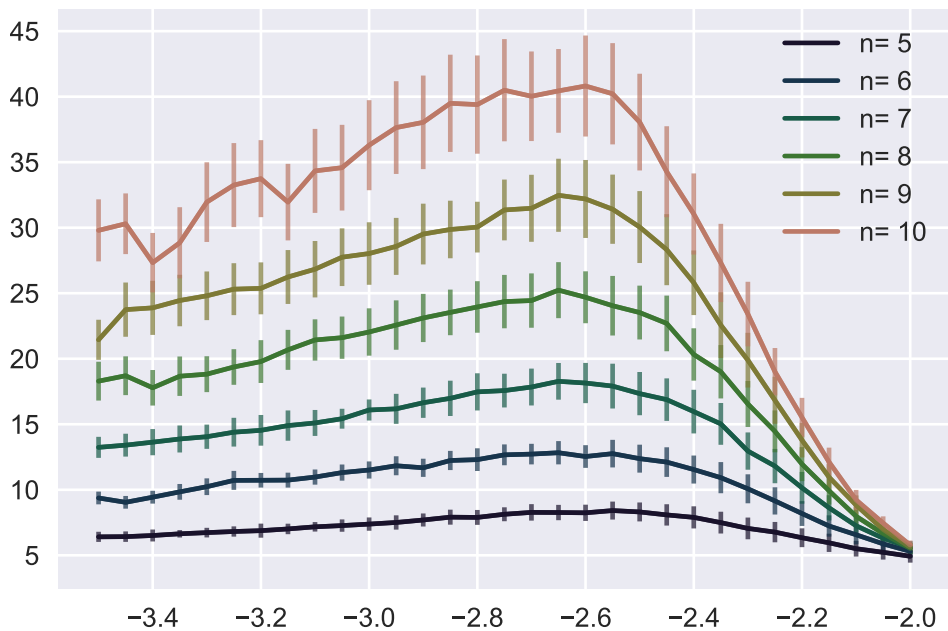
Planck Normalised Volumes for type 11 scaled by d=\max V
